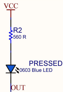
BUTTON LED
