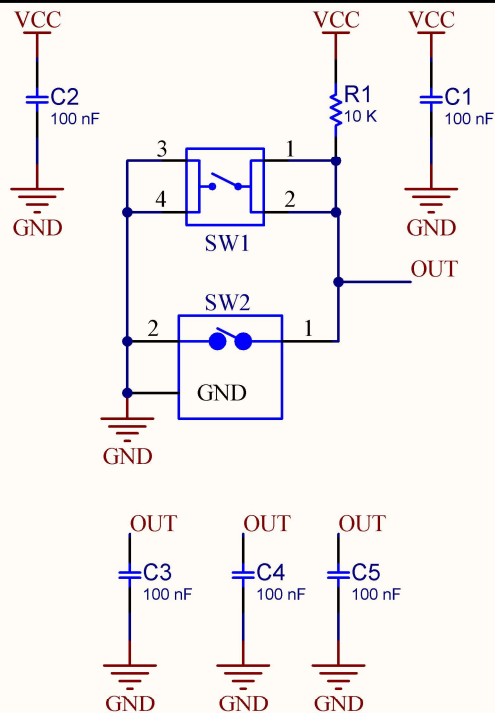
BUTTON CIRCUIT
