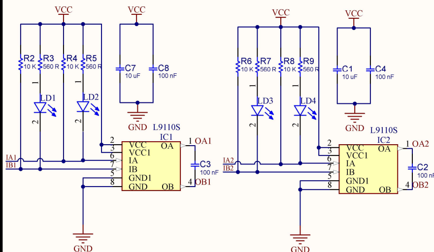
L9110S
