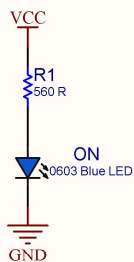
POWER LED
